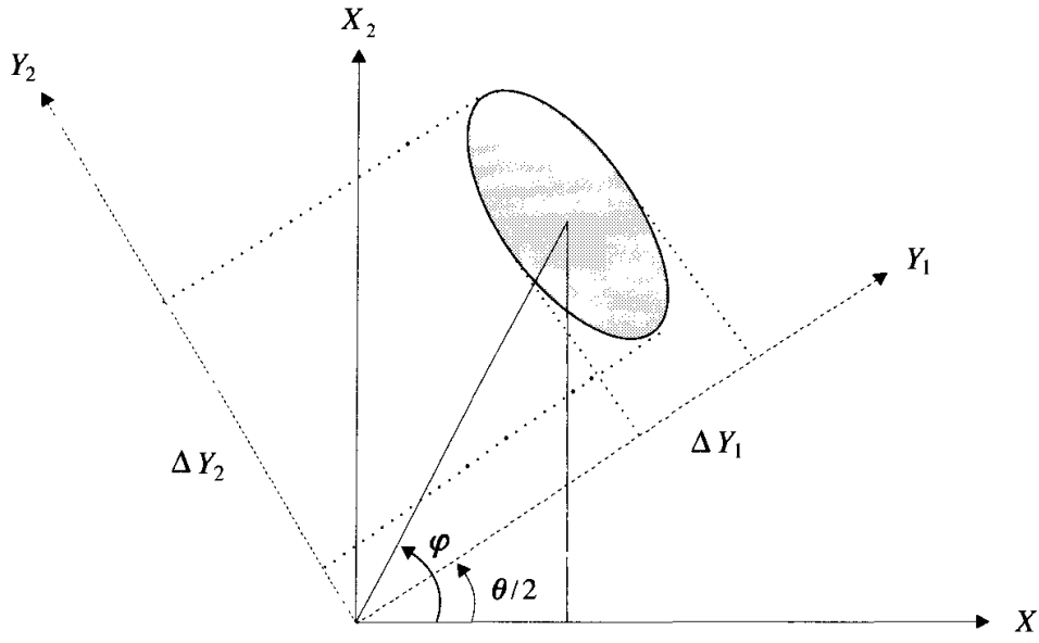
Fig. 2.8 Error contour for a squeezed coherent state.
