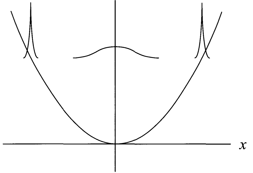
Fig. 2.3 Evolution of a squeezed state of a simple harmonic oscillator.
